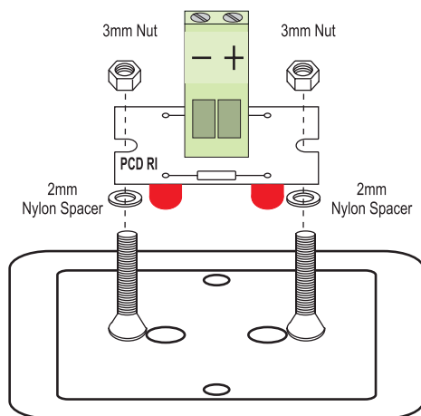
Back View With PCB Mounting Detail
