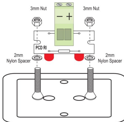
Back View With PCB Mounting Detail
