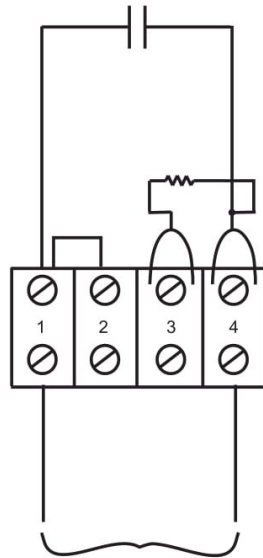
Zone Terminals of the Fire Alarm Panel
