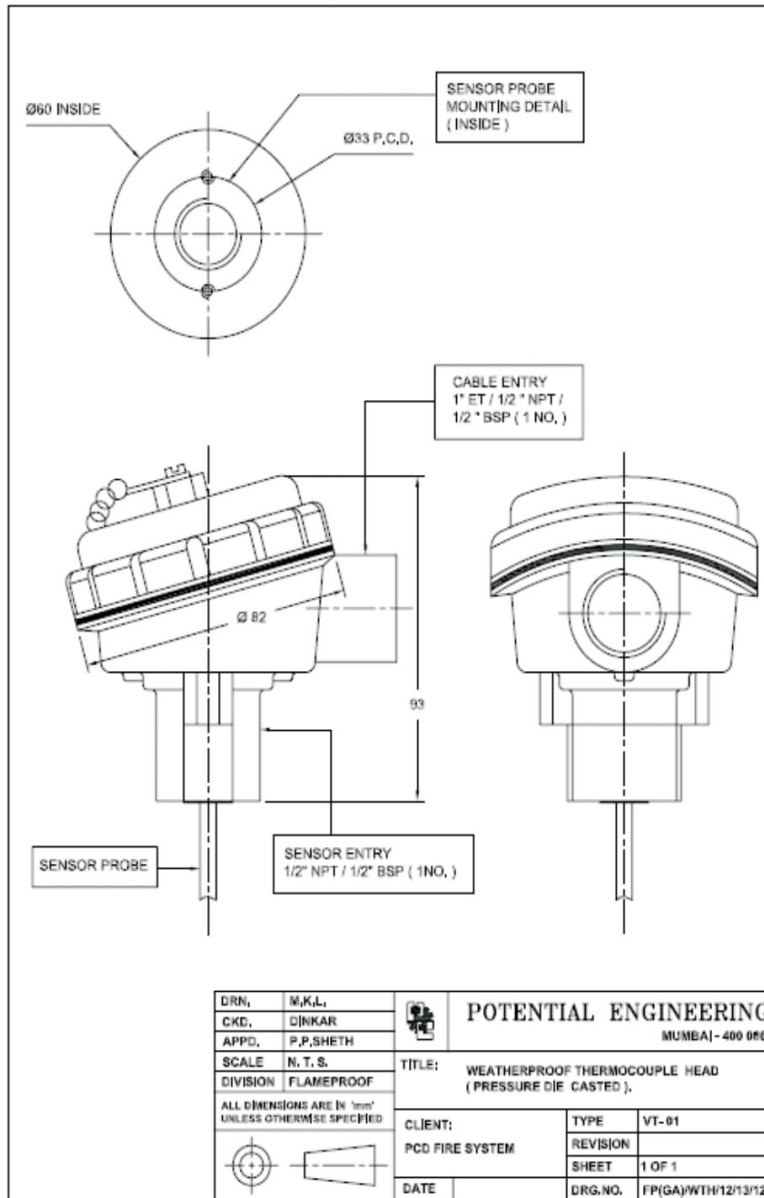
Thermocouple Head Dimensions
